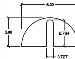
MOUNTING SLOT DETAIL SCALE 2:1 ALL DIMS NOMINAL
