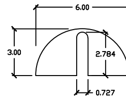
MOUNTING SLOT DETAIL SCALE 2:1
