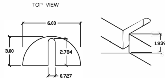
MOUNTING SLOT DETAIL SCALE 2:1 ALL DIMS NOMINAL
