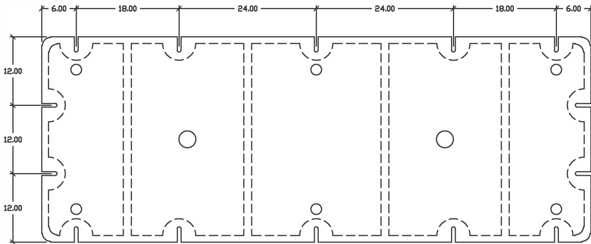
MOUNTING SLOT DETAIL SCALE 2:1
