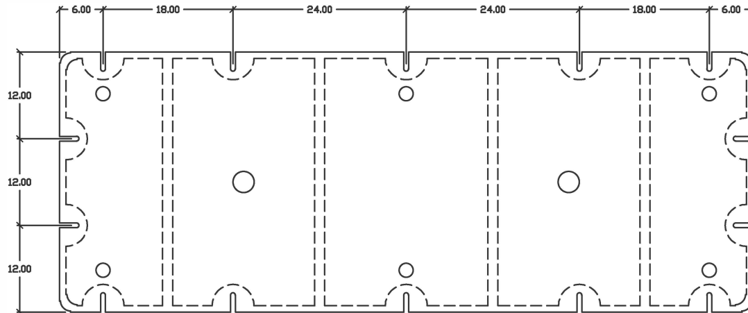
MOUNTING SLOT DETAIL SCALE 2:1
