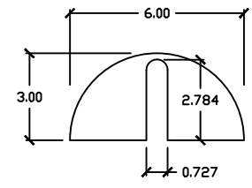
MOUNTING SLOT DETAIL SCALE 2:1 ALL DIMS NOMINAL
