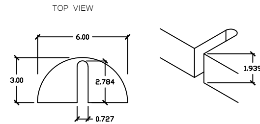
MOUNTING SLOT DETAIL SCALE 2:1 ALL DIMS NOMINAL
