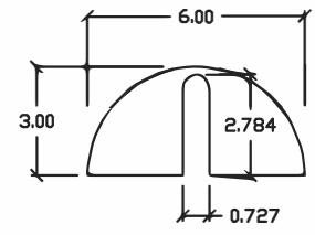
MOUNTING SLOT DETAIL SCALE 2:1
