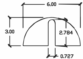
MOUNTING SLOT DETAIL SCALE 2:1 ALL DIMS NOMINAL
