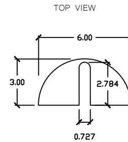
MOUNTING SLOT DETAIL SCALE 2:1
