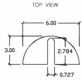
MOUNTING SLOT DETAIL SCALE 2:1
