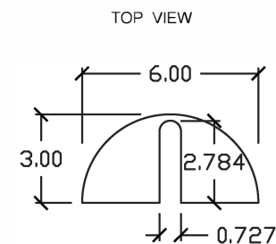
MOUNTING SLOT DETAIL SCALE 2:1
